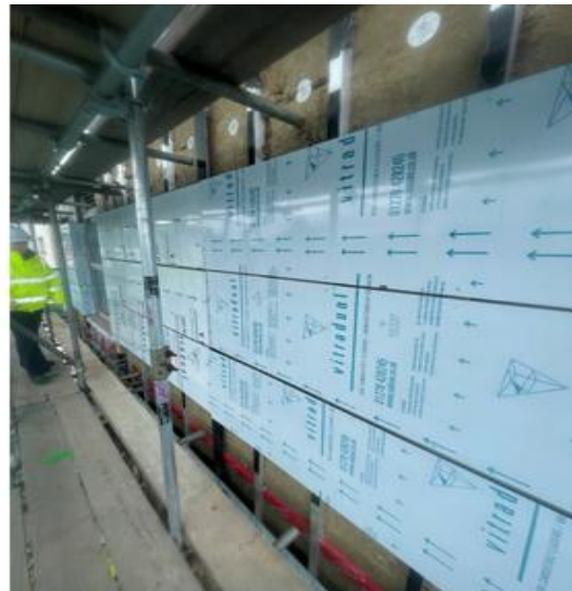
Picture showing panels temporarily fixed onto sub structure – being inspected by QA
